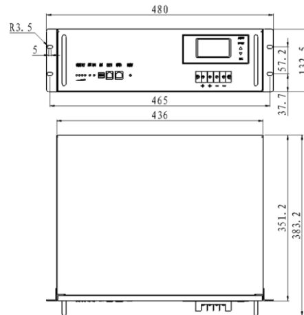
Figure 3 Battery Size
